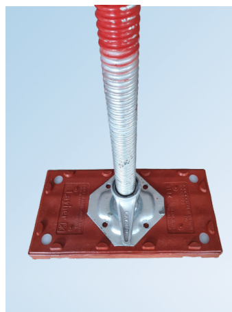
Appui central
